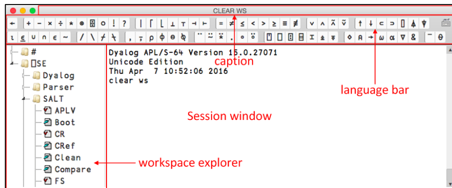
Figure 7. The Dyalog Session user interface with workspace explorer – Mac OS
