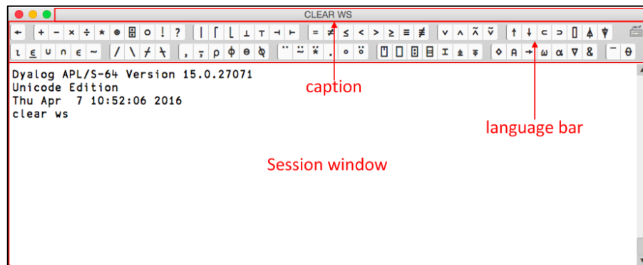
Figure 6. The Dyalog Session user interface (default) – Mac OS
