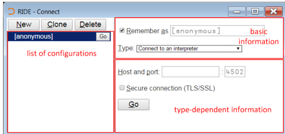
Figure 1. Areas of the RIDE - Connect dialog box – Microsoft Windows
